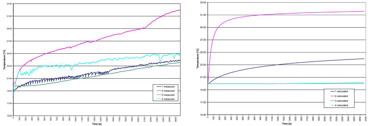
Fig.2 Temperature evolution
