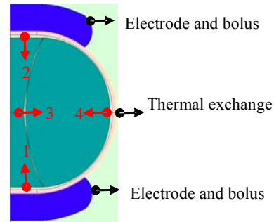
Fig.1b 2D geometric model for FEM analysis
